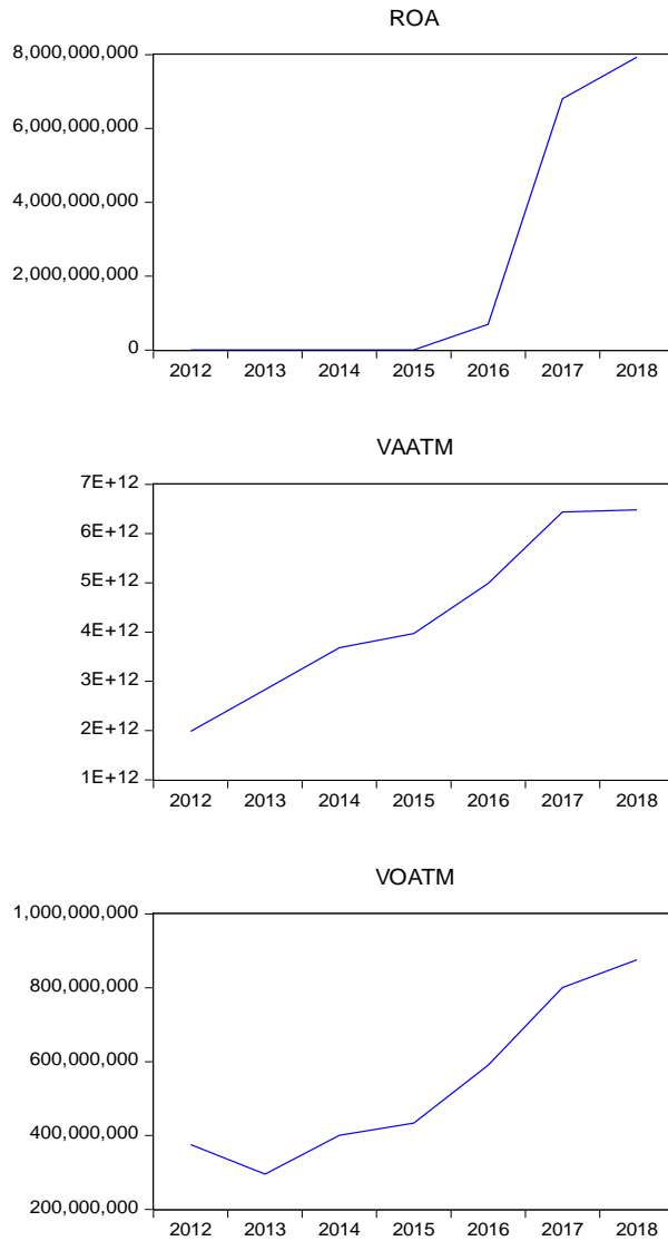
Figure 1: Trend analysis
